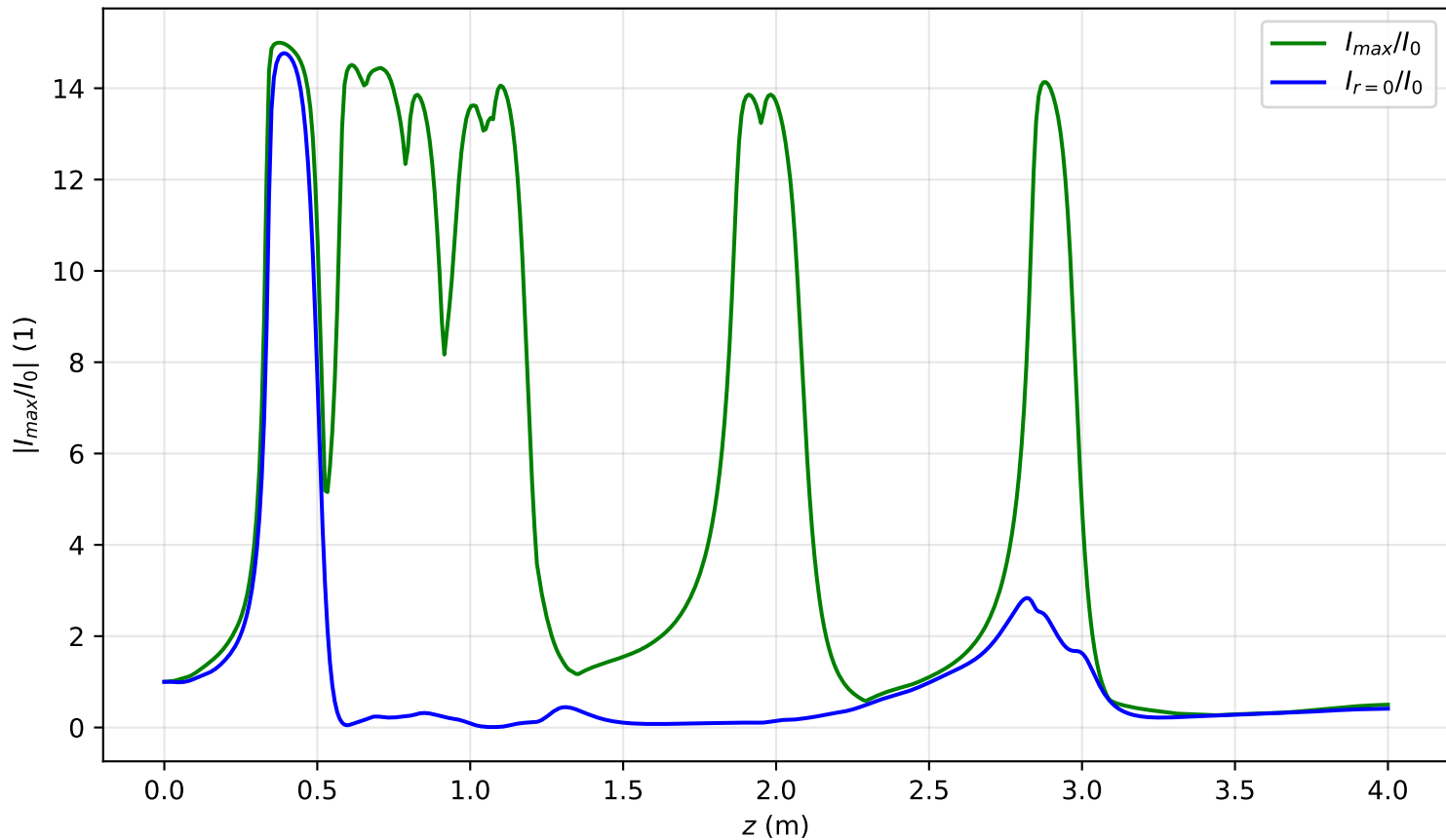
I_{max}(x=0, y=0, z)/I_0 , Pin=7.4Pcr, noisy input, artificial time
